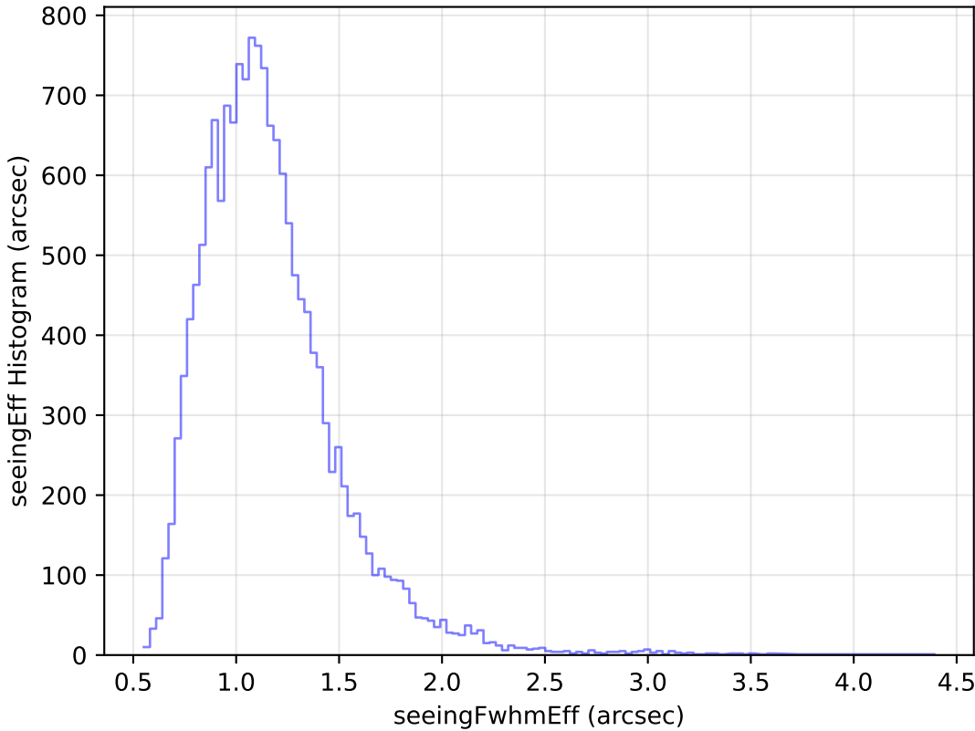
ddf_loaded_half_fl8_v3.4_10yrs Yr 1 u band: seeingEff Histogram
