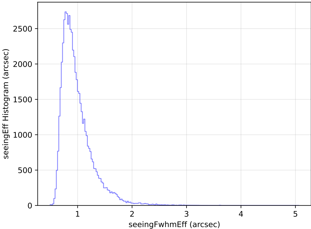
ddf_loaded_half_fl8_v3.4_10yrs Yr 1 i band: seeingEff Histogram
