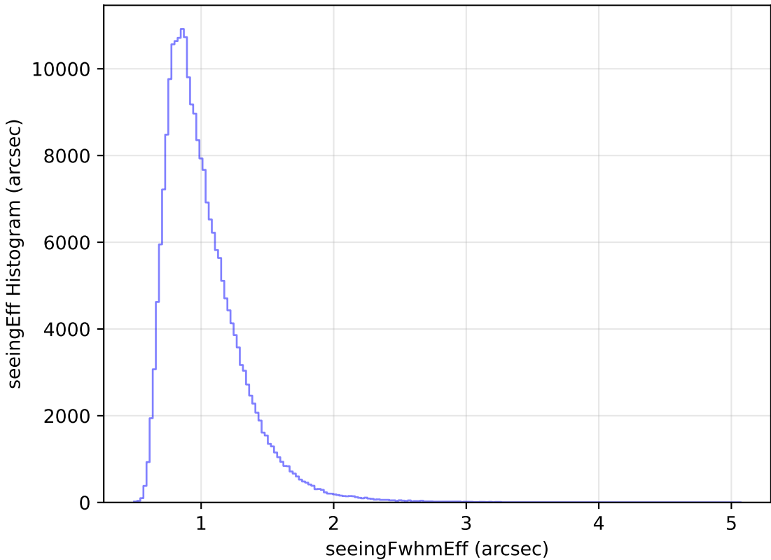
ddf_loaded_half_fl8_v3.4_10yrs Yr 1 all bands: seeingEff Histogram
