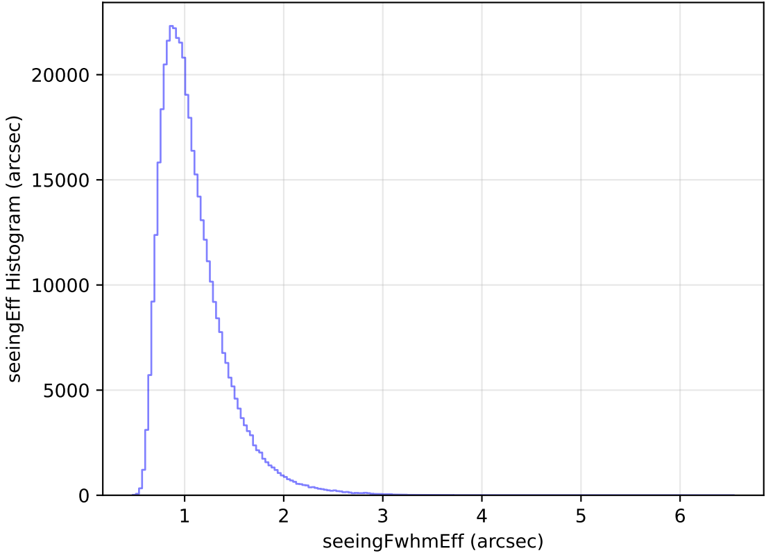
ddf_loaded_half_fl8_v3.4_10yrs WFD z band: seeingEff Histogram
