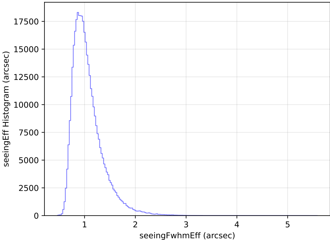
ddf_loaded_half_fl8_v3.4_10yrs WFD y band: seeingEff Histogram
