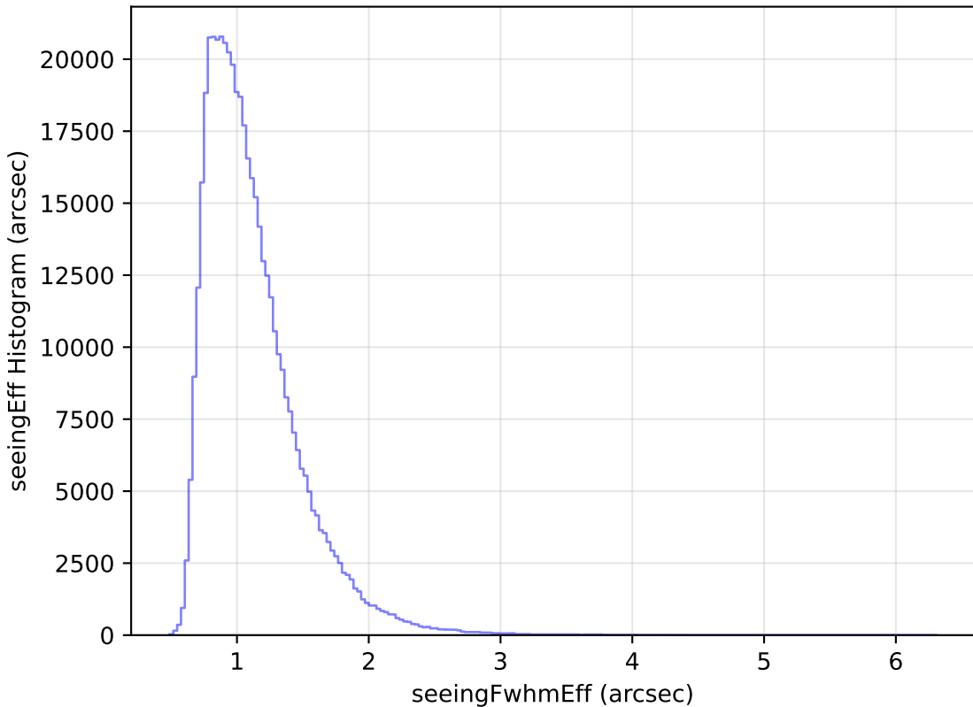
ddf_loaded_half_fl8_v3.4_10yrs WFD r band: seeingEff Histogram
