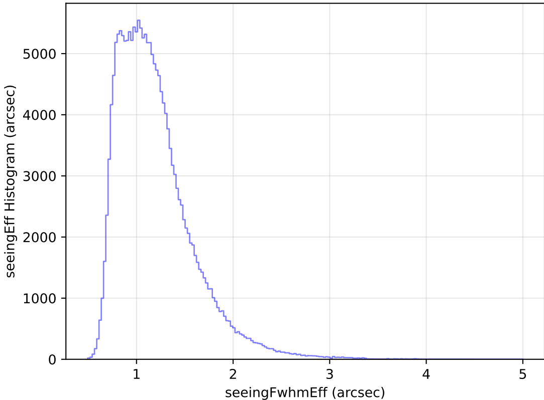
ddf_loaded_half_fl8_v3.4_10yrs WFD g band: seeingEff Histogram
