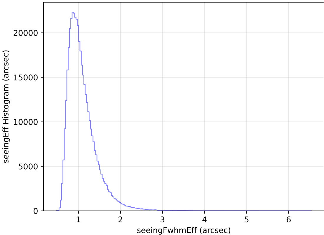
ddf_loaded_half_fl8_v3.4_10yrs All sky z band: seeingEff Histogram
