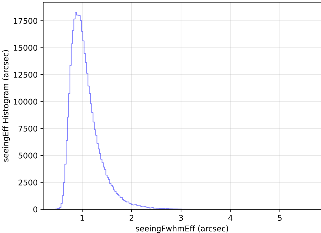
ddf_loaded_half_fl8_v3.4_10yrs All sky y band: seeingEff Histogram
