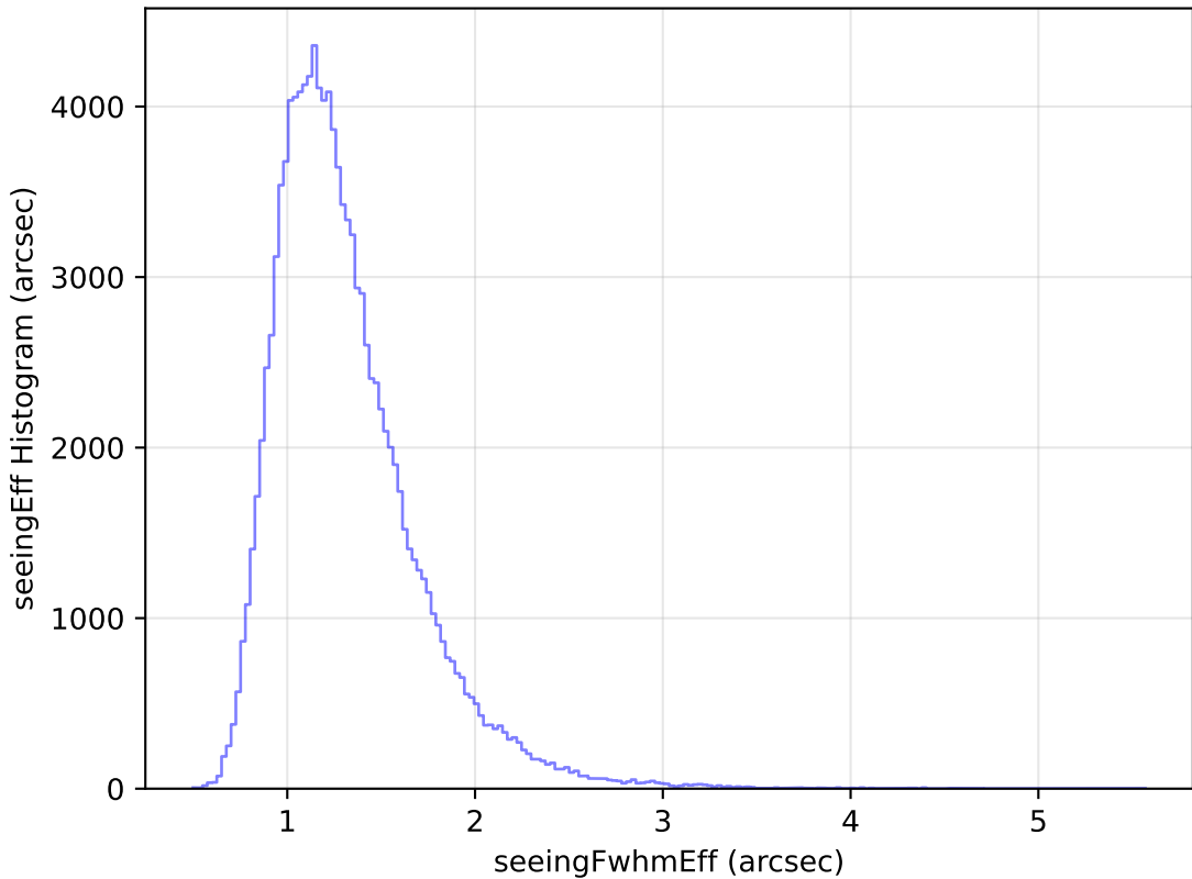
ddf_loaded_half_fl8_v3.4_10yrs All sky u band: seeingEff Histogram
