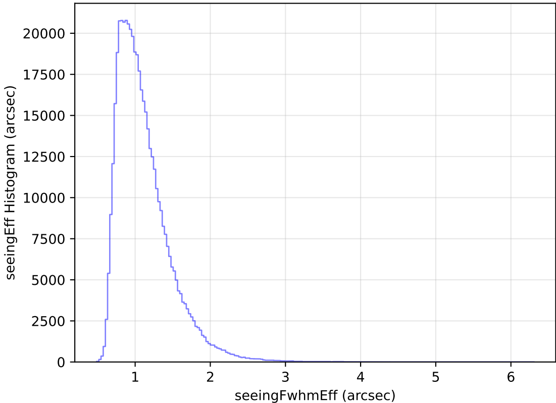
ddf_loaded_half_fl8_v3.4_10yrs All sky r band: seeingEff Histogram
