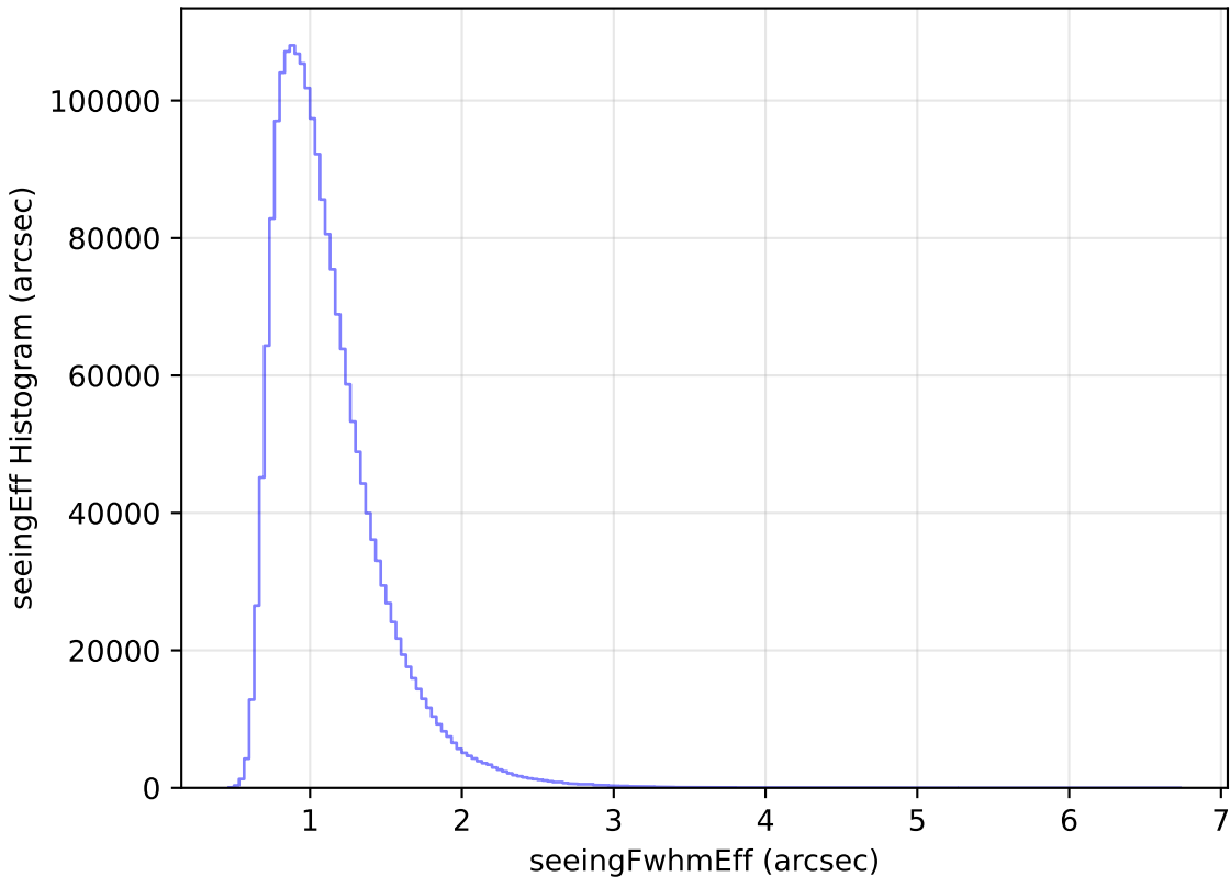
ddf_loaded_half_fl8_v3.4_10yrs All sky all bands: seeingEff Histogram
