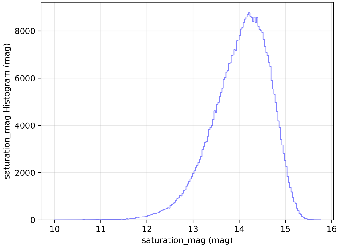
ddf_loaded_half_fl8_v3.4_10yrs WFD z band: saturation_mag Histogram
