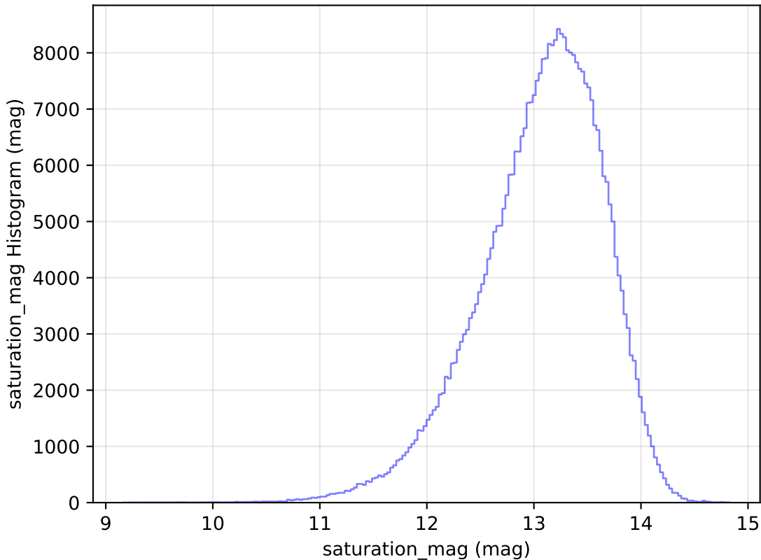
ddf_loaded_half_fl8_v3.4_10yrs WFD y band: saturation_mag Histogram
