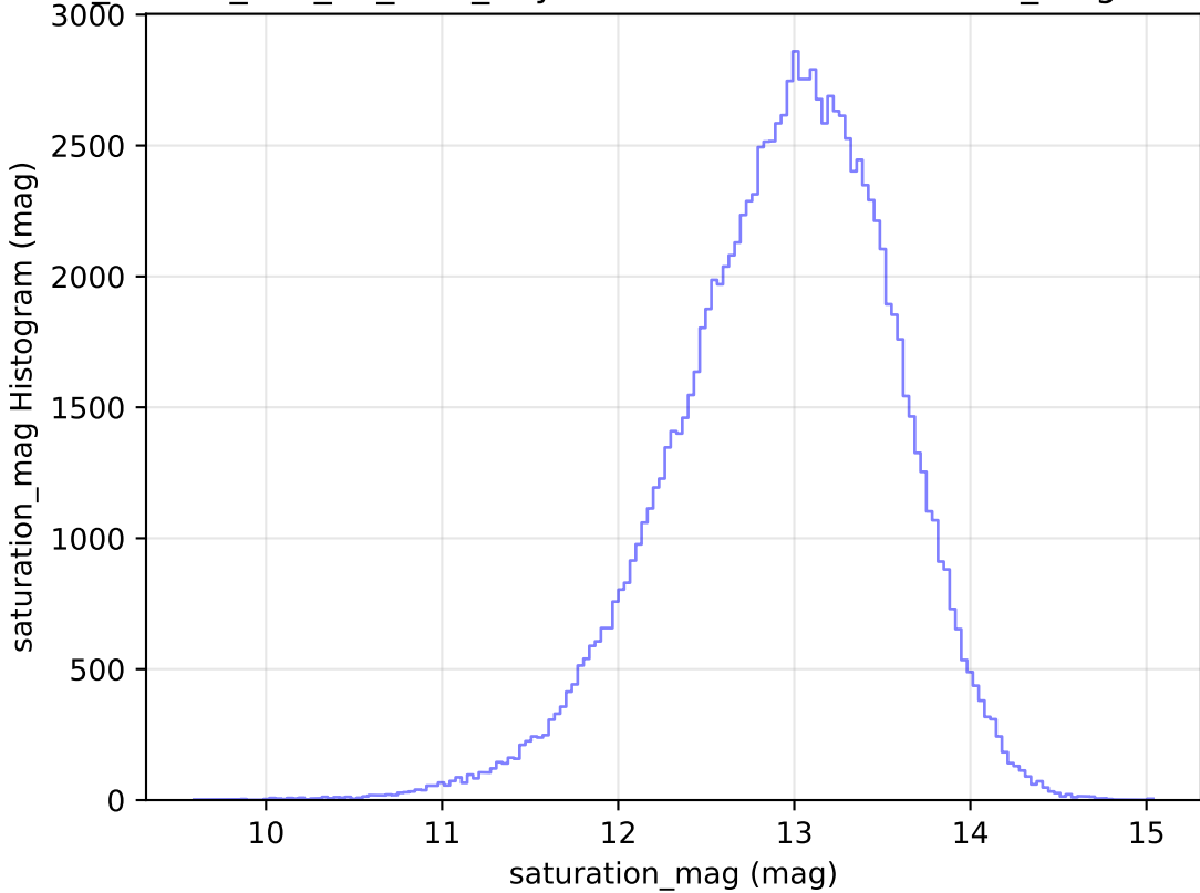
ddf_loaded_half_fl8_v3.4_10yrs WFD u band: saturation_mag Histogram
