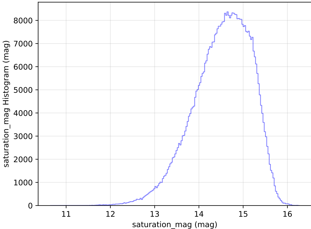
ddf_loaded_half_fl8_v3.4_10yrs WFD r band: saturation_mag Histogram
