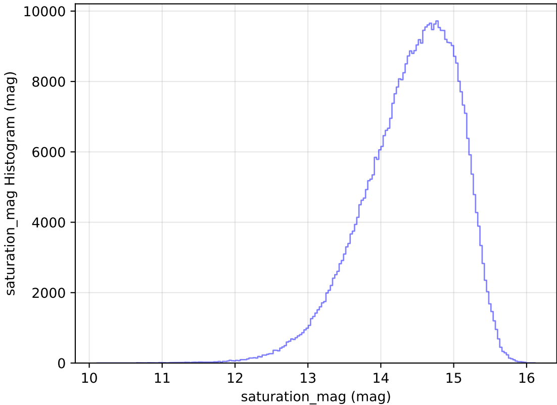
ddf_loaded_half_fl8_v3.4_10yrs WFD i band: saturation_mag Histogram
