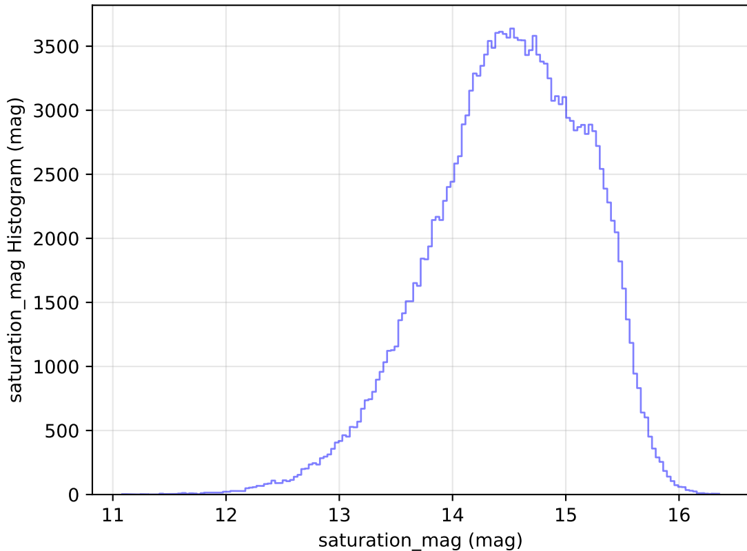
ddf_loaded_half_fl8_v3.4_10yrs WFD g band: saturation_mag Histogram
