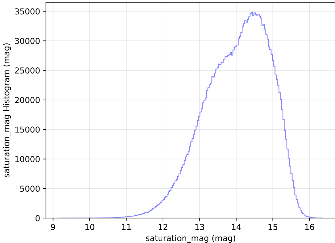
ddf_loaded_half_fl8_v3.4_10yrs WFD all bands: saturation_mag Histogram
