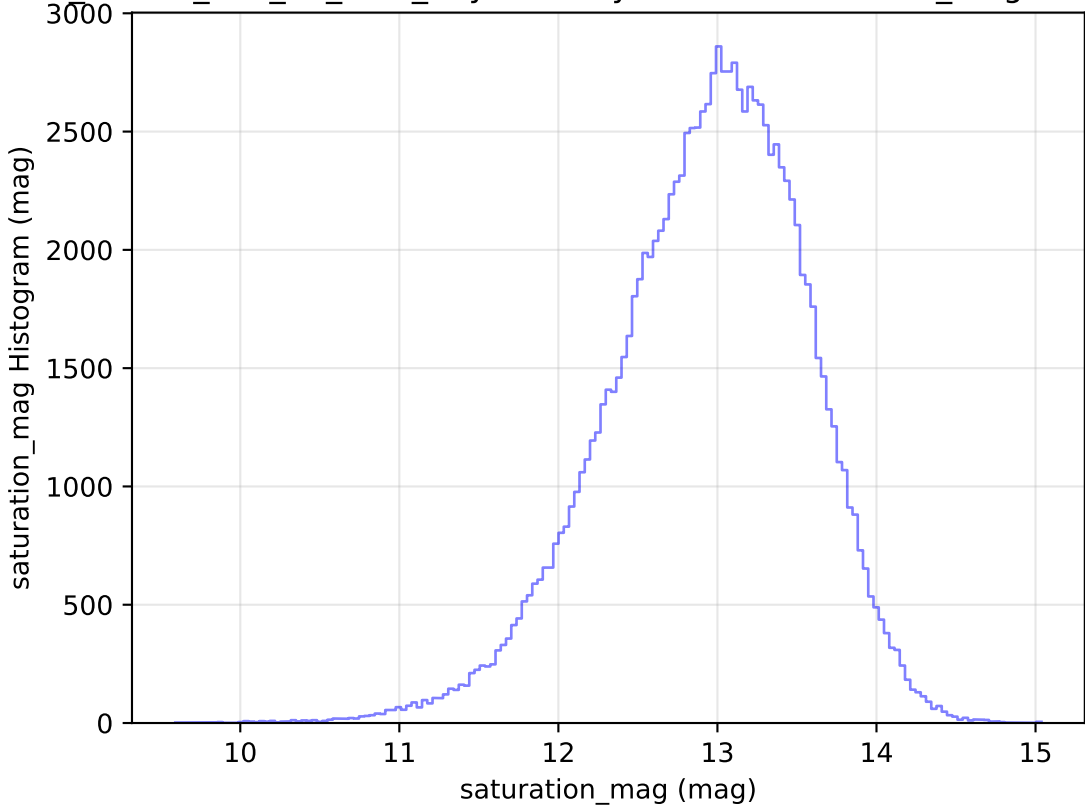
ddf_loaded_half_fl8_v3.4_10yrs All sky u band: saturation_mag Histogram
