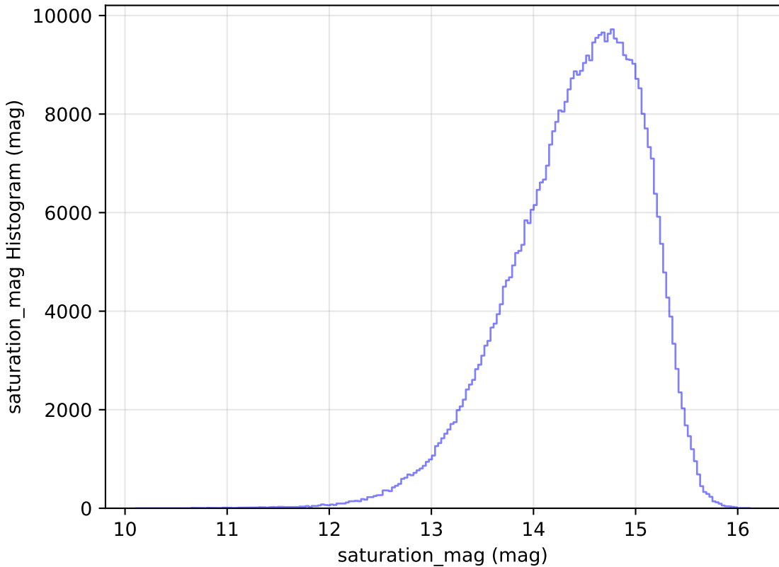
ddf_loaded_half_fl8_v3.4_10yrs All sky i band: saturation_mag Histogram
