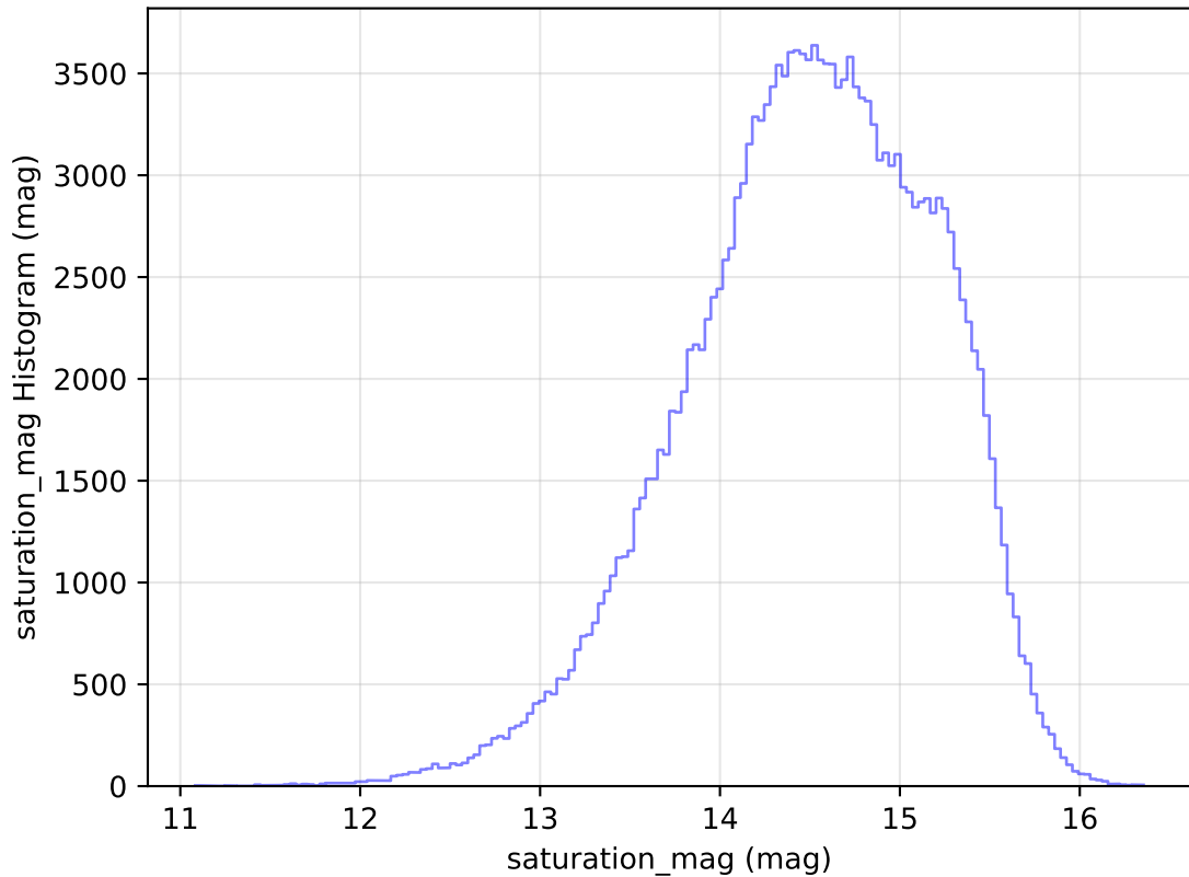
ddf_loaded_half_fl8_v3.4_10yrs All sky g band: saturation_mag Histogram
