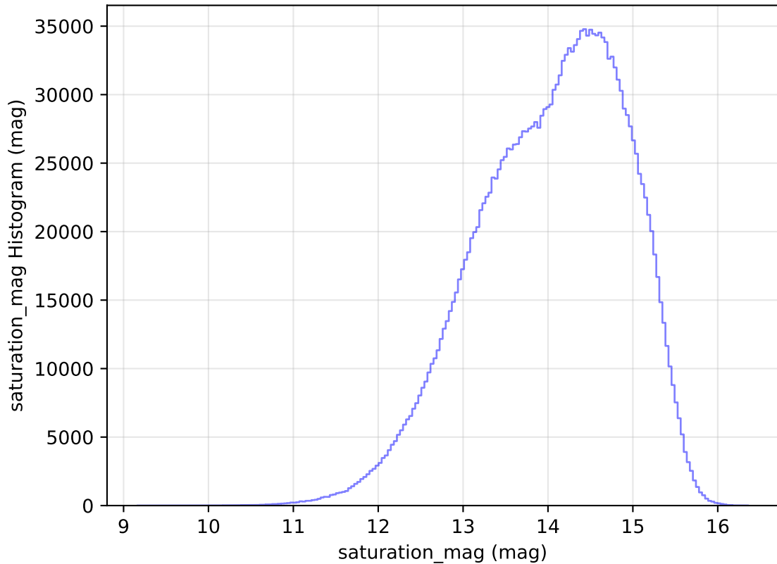
ddf_loaded_half_fl8_v3.4_10yrs All sky all bands: saturation_mag Histogram
