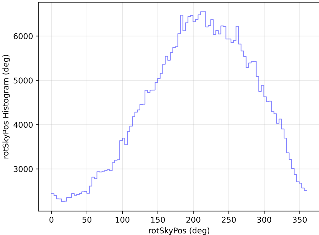
ddf_loaded_half_fl8_v3.4_10yrs WFD z band: rotSkyPos Histogram
