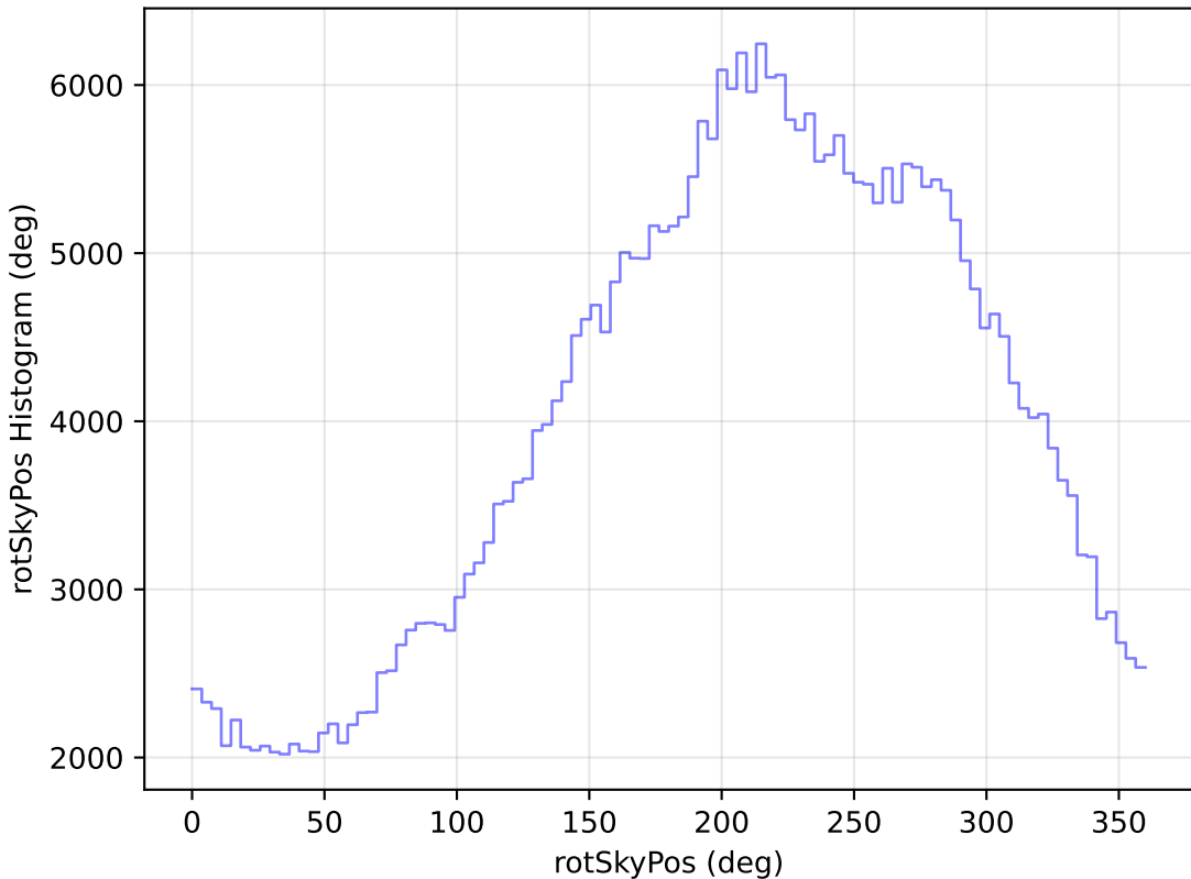
ddf_loaded_half_fl8_v3.4_10yrs WFD y band: rotSkyPos Histogram
