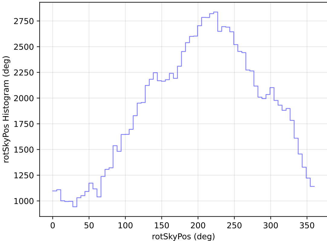
ddf_loaded_half_fl8_v3.4_10yrs WFD u band: rotSkyPos Histogram
