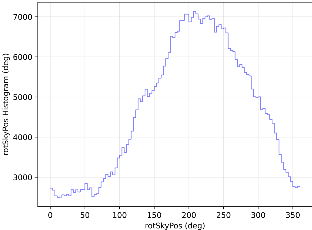
ddf_loaded_half_fl8_v3.4_10yrs WFD i band: rotSkyPos Histogram
