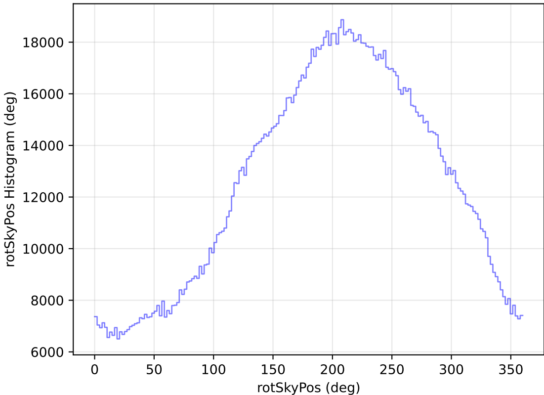
ddf_loaded_half_fl8_v3.4_10yrs WFD all bands: rotSkyPos Histogram
