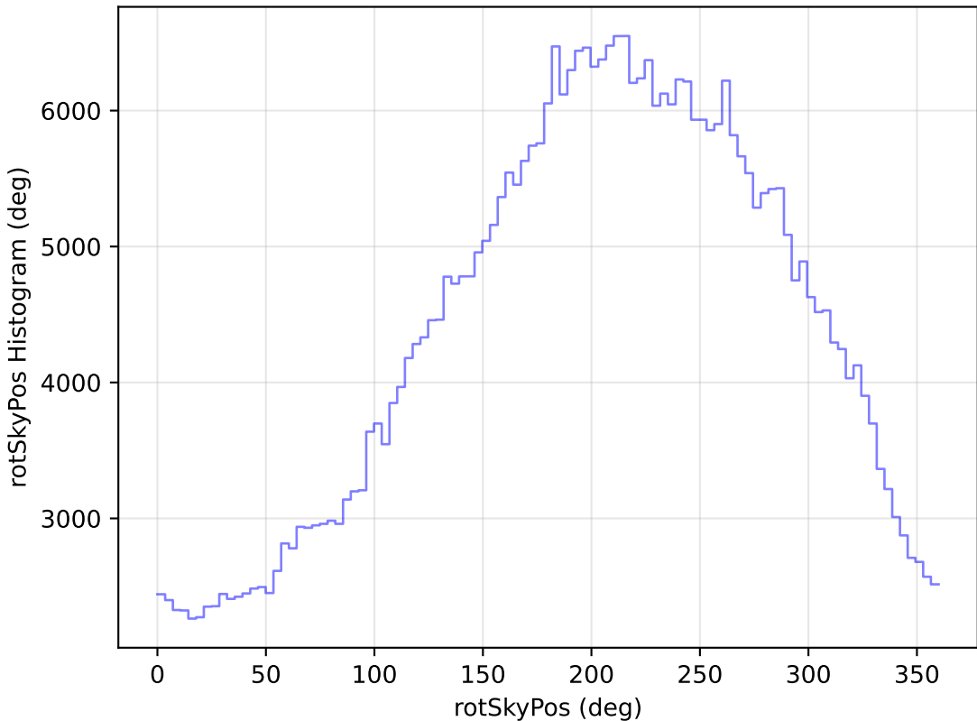
ddf_loaded_half_fl8_v3.4_10yrs All sky z band: rotSkyPos Histogram
