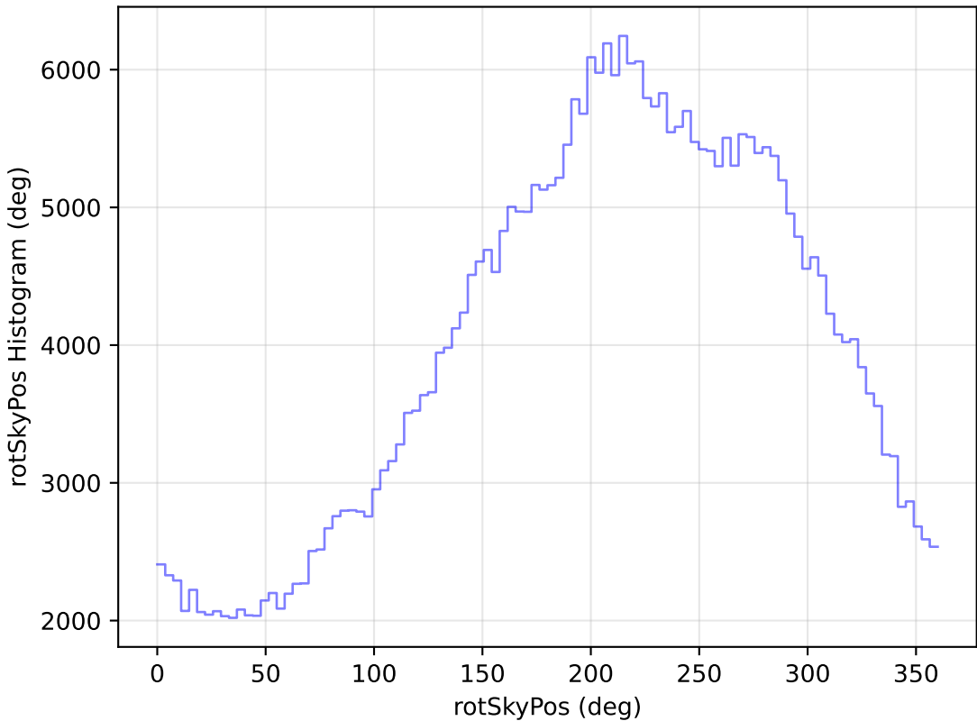
ddf_loaded_half_fl8_v3.4_10yrs All sky y band: rotSkyPos Histogram
