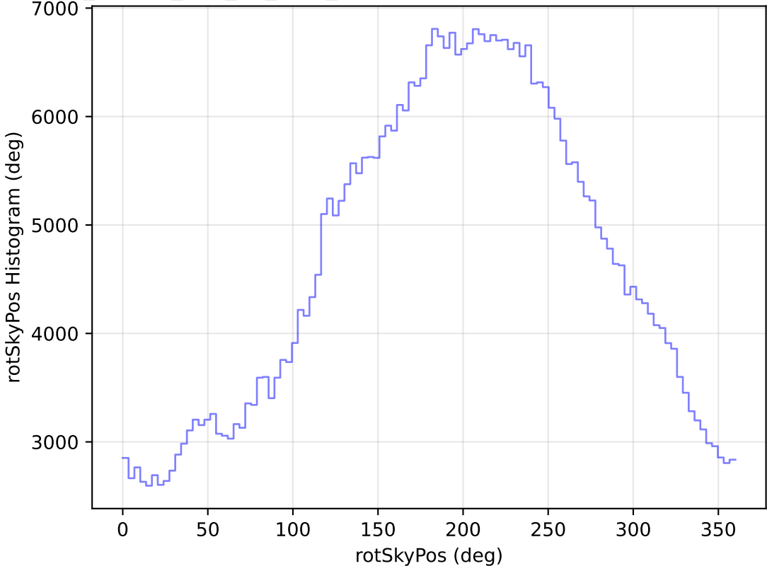
ddf_loaded_half_fl8_v3.4_10yrs All sky r band: rotSkyPos Histogram
