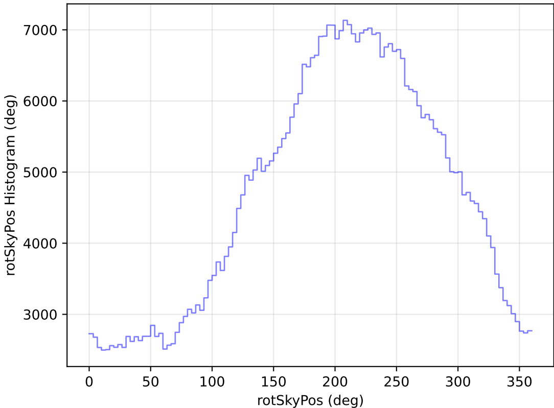
ddf_loaded_half_fl8_v3.4_10yrs All sky i band: rotSkyPos Histogram
