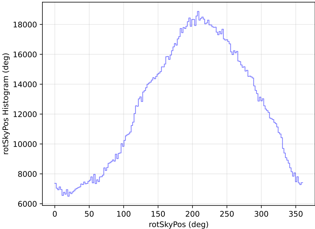
ddf_loaded_half_fl8_v3.4_10yrs All sky all bands: rotSkyPos Histogram
