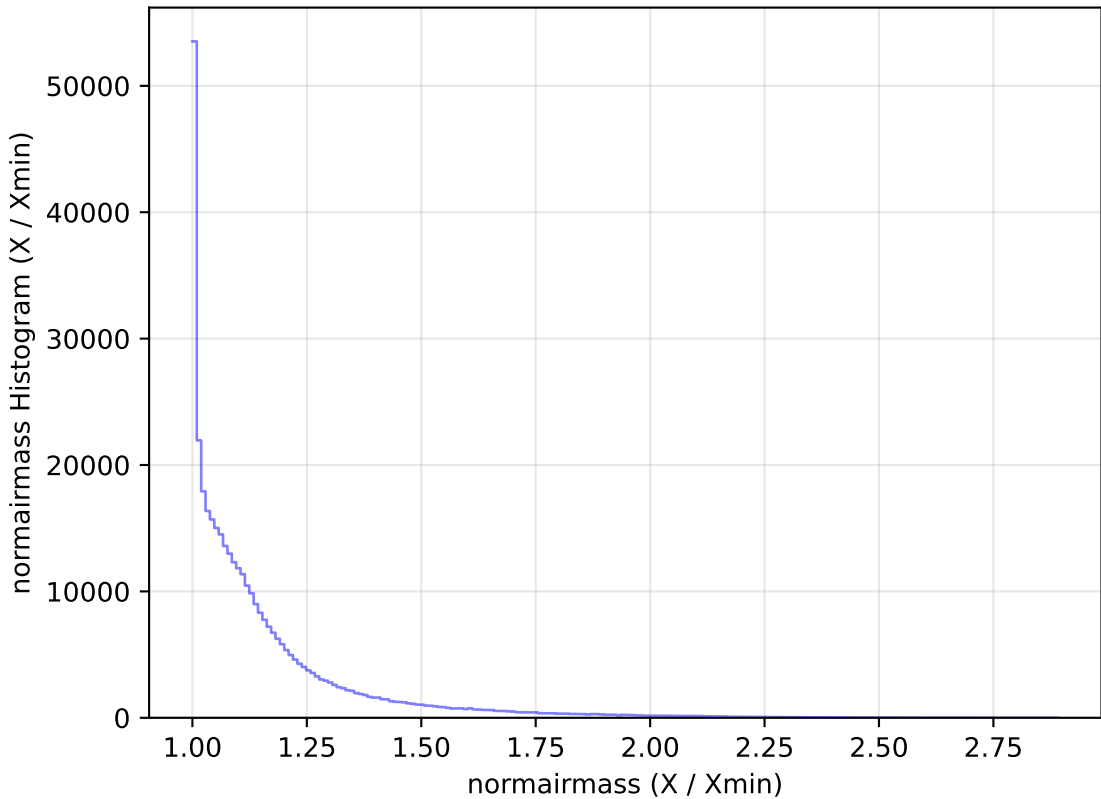
ddf_loaded_half_fl8_v3.4_10yrs WFD y band: normairmass Histogram
