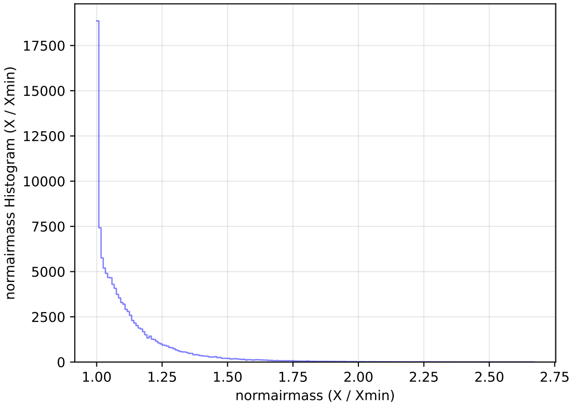
ddf_loaded_half_fl8_v3.4_10yrs WFD u band: normairmass Histogram
