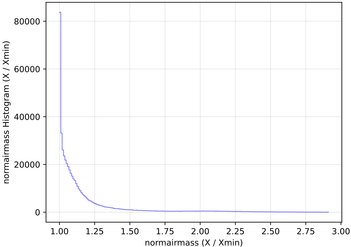
ddf_loaded_half_fl8_v3.4_10yrs WFD i band: normairmass Histogram
