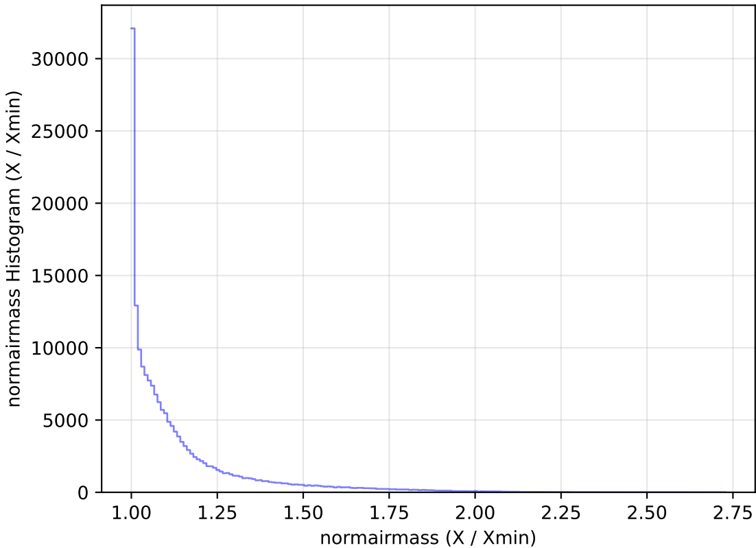
ddf_loaded_half_fl8_v3.4_10yrs WFD g band: normairmass Histogram
