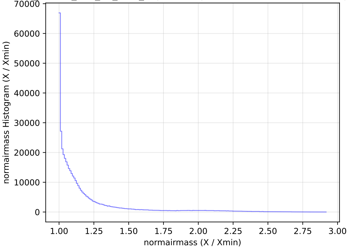
ddf_loaded_half_fl8_v3.4_10yrs All sky z band: normairmass Histogram
