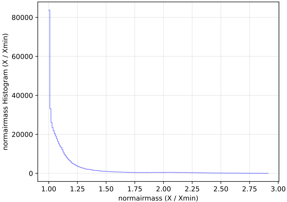
ddf_loaded_half_fl8_v3.4_10yrs All sky i band: normairmass Histogram
