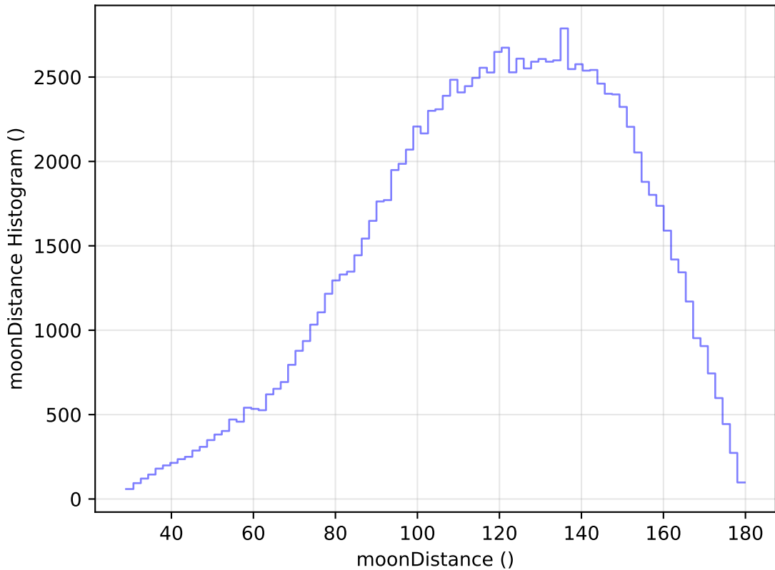
ddf_loaded_half_fl8_v3.4_10yrs WFD u band: moonDistance Histogram
