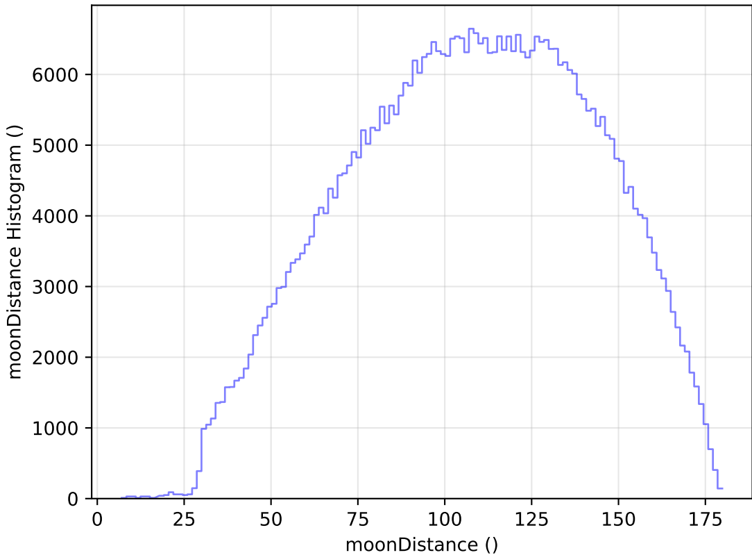
ddf_loaded_half_fl8_v3.4_10yrs WFD r band: moonDistance Histogram
