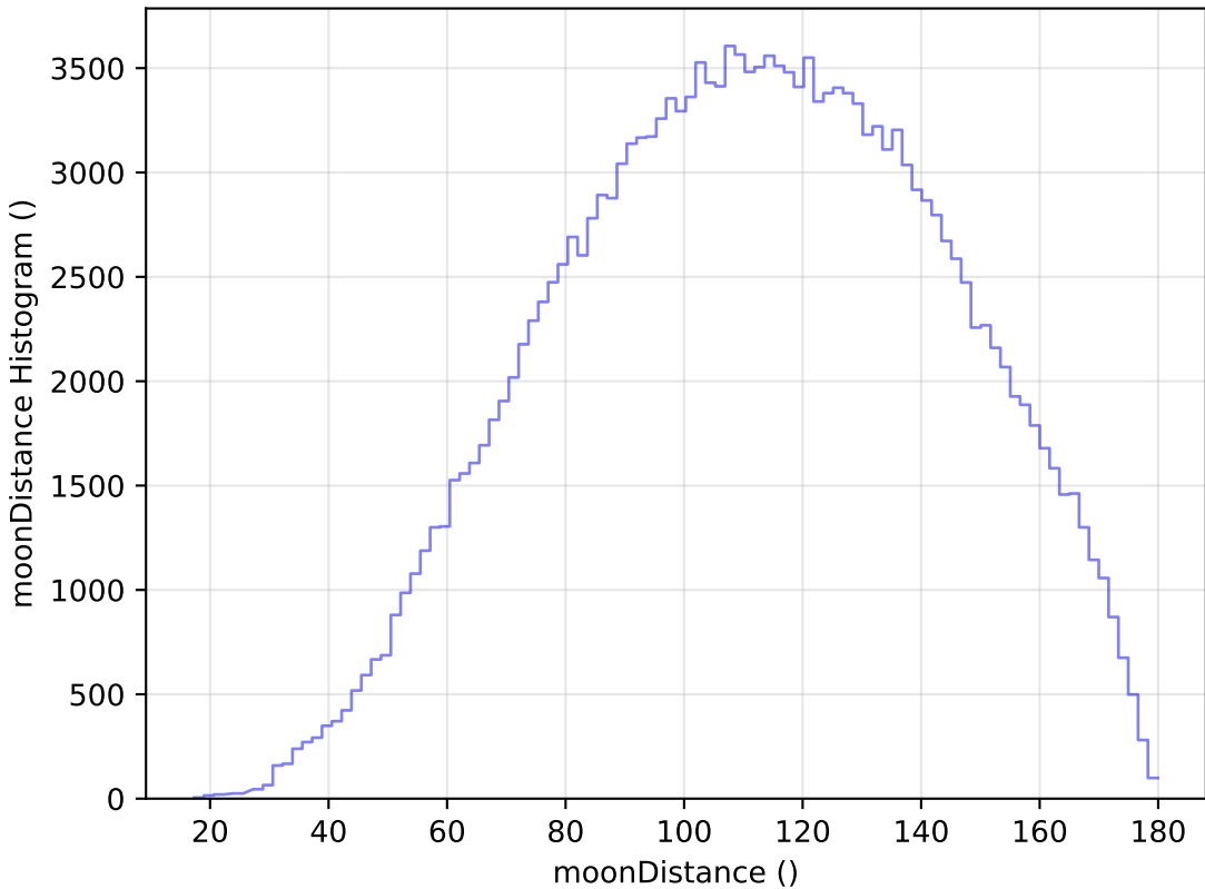
ddf_loaded_half_fl8_v3.4_10yrs WFD g band: moonDistance Histogram
