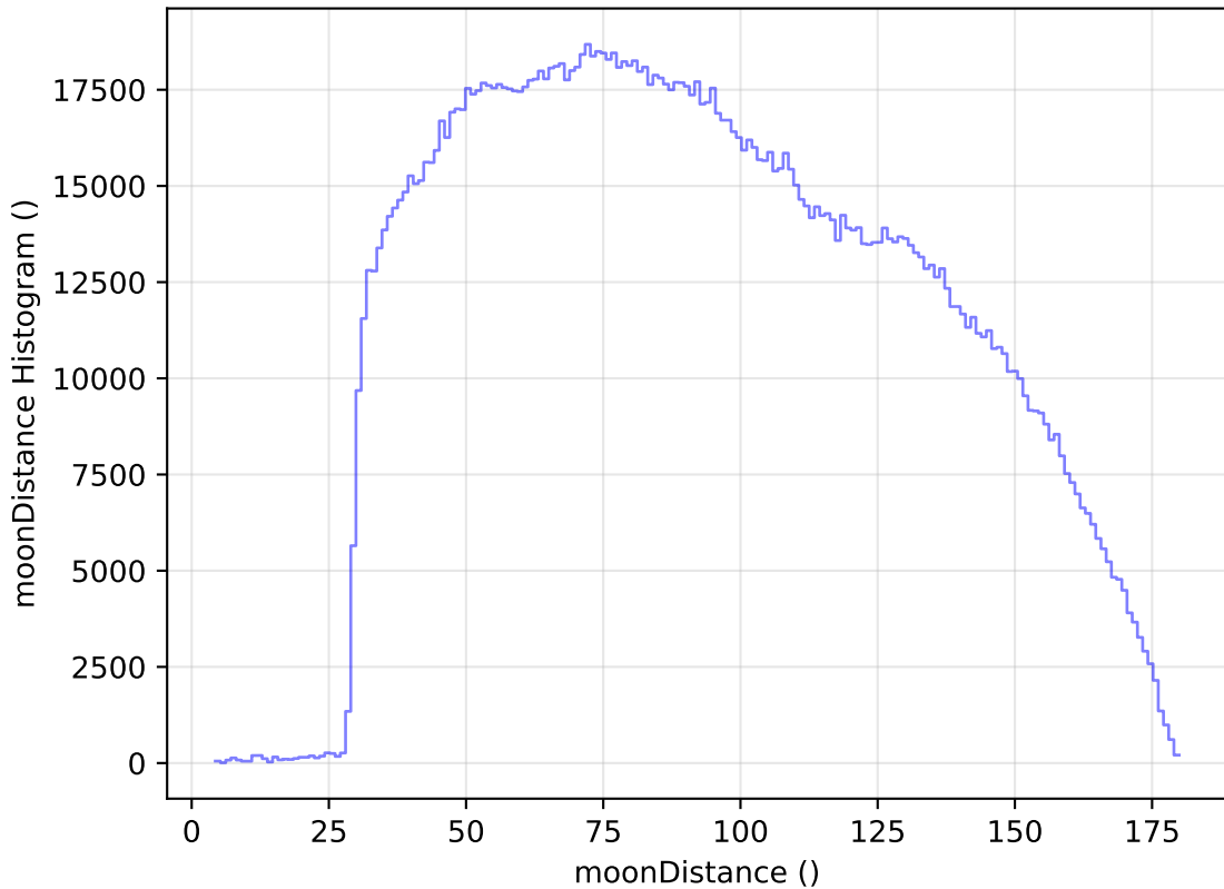
ddf_loaded_half_fl8_v3.4_10yrs WFD all bands: moonDistance Histogram
