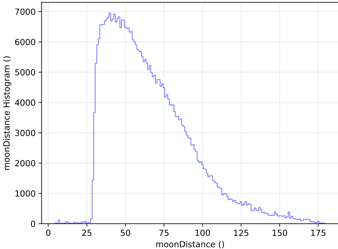
ddf_loaded_half_fl8_v3.4_10yrs All sky y band: moonDistance Histogram
