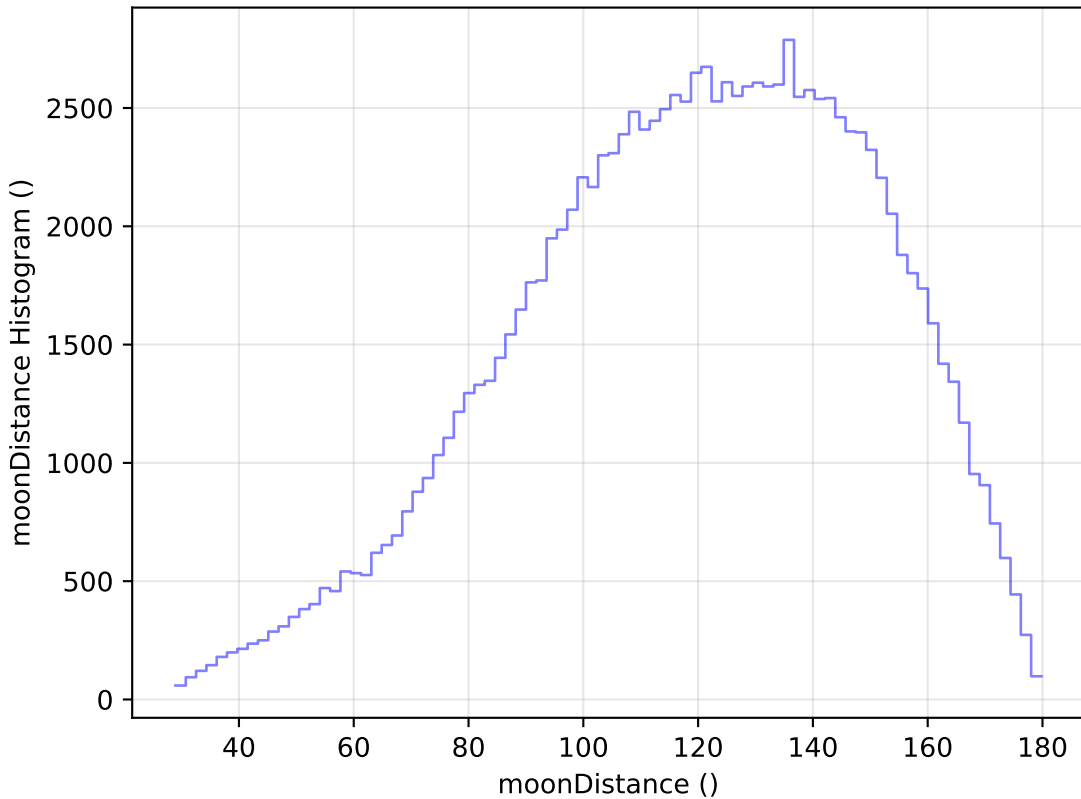
ddf_loaded_half_fl8_v3.4_10yrs All sky u band: moonDistance Histogram
