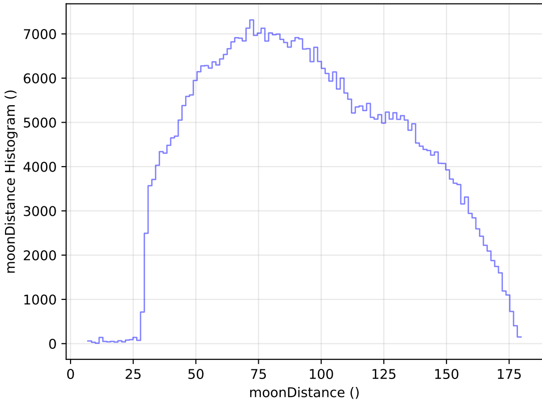
ddf_loaded_half_fl8_v3.4_10yrs All sky i band: moonDistance Histogram
