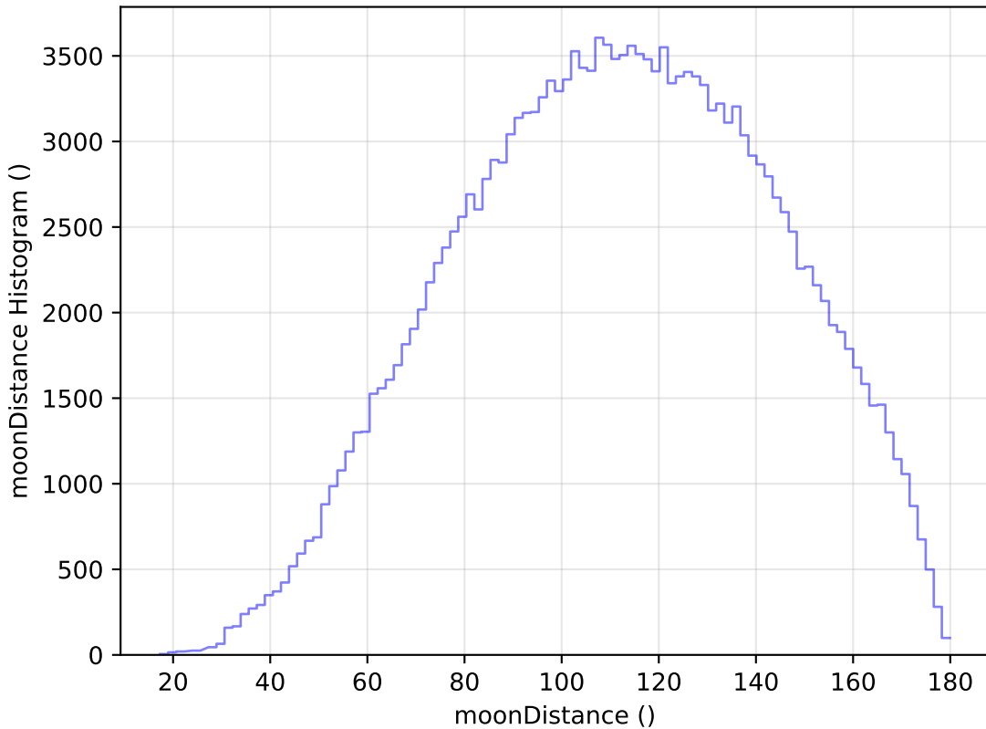
ddf_loaded_half_fl8_v3.4_10yrs All sky g band: moonDistance Histogram
