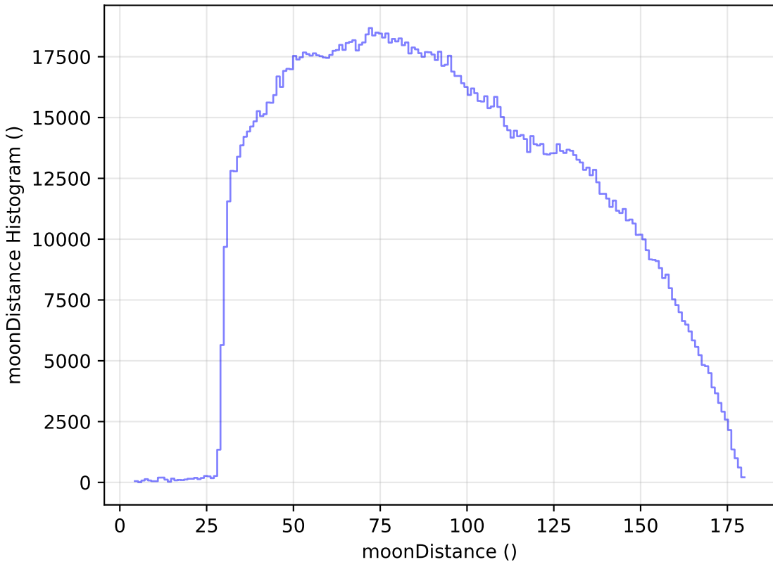
ddf_loaded_half_fl8_v3.4_10yrs All sky all bands: moonDistance Histogram
