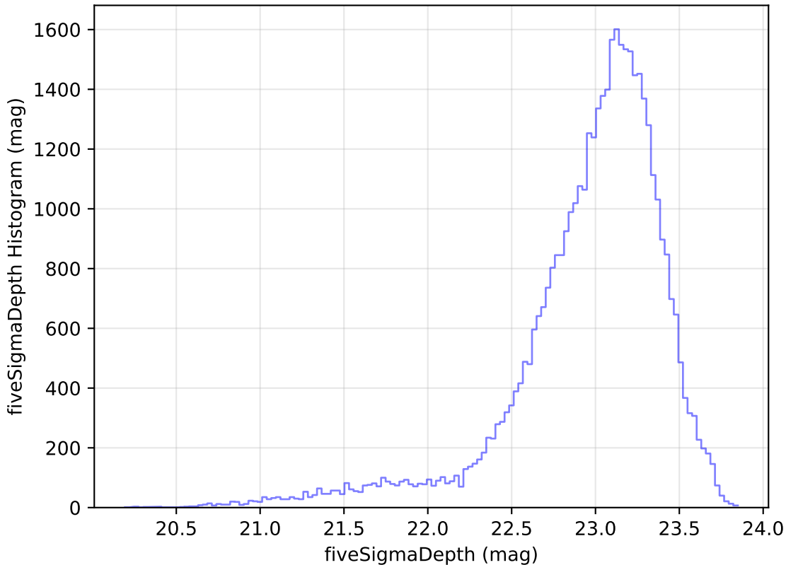
ddf_loaded_half_fl8_v3.4_10yrs Yr 1 z band: fiveSigmaDepth Histogram
