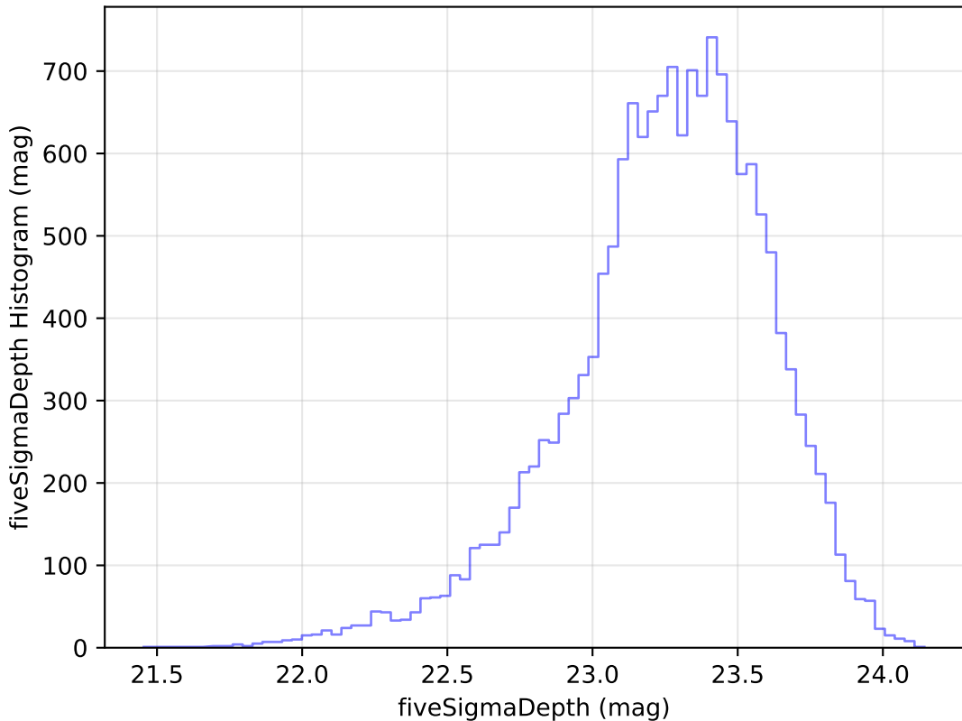
ddf_loaded_half_fl8_v3.4_10yrs Yr 1 u band: fiveSigmaDepth Histogram
